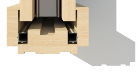
BLIND PARTITION WITH UPRIGHT
